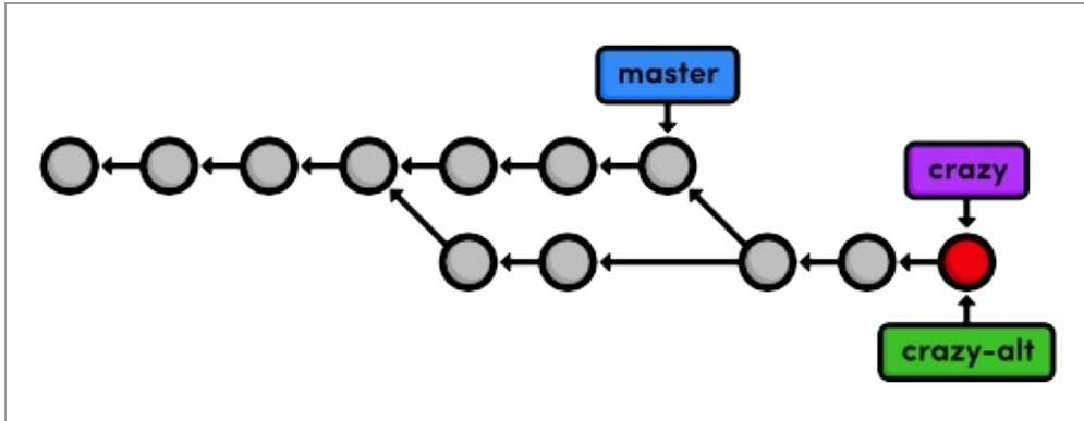
Creating the crazy-alt branch
