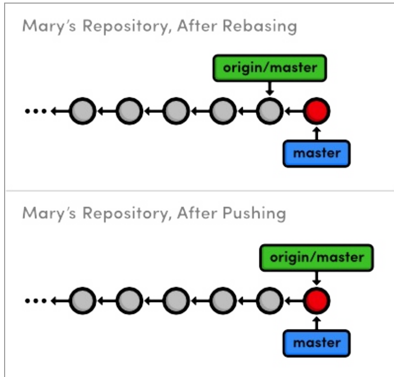
Updating the central repository's master
