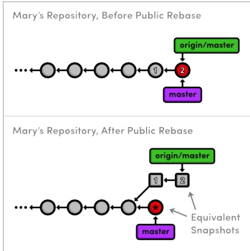
Squashing a public commit
