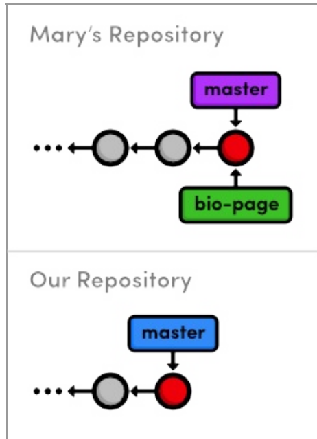
Merging Mary's bio-page branch with her master
